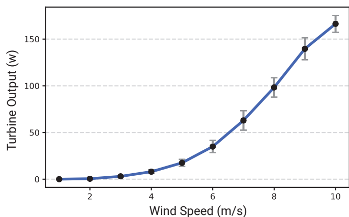
CW 100 Power Curve
