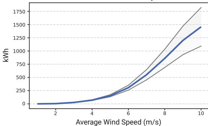
Annual CW100 Output
